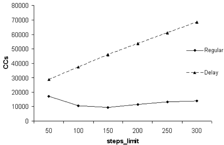
Figure 21: Number of non-concurrent constraint checks performed by ConcDB for a smaller range of steps_limits ( p_1 = 0.4 )
