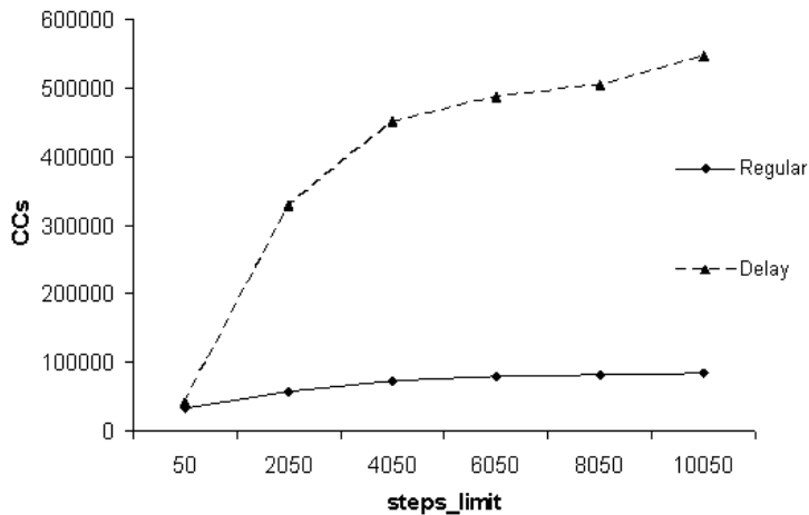
Figure 20: Number of non-concurrent constraint checks performed by ConcDB for increasing steps_limits ( p_1 = 0.7 )
