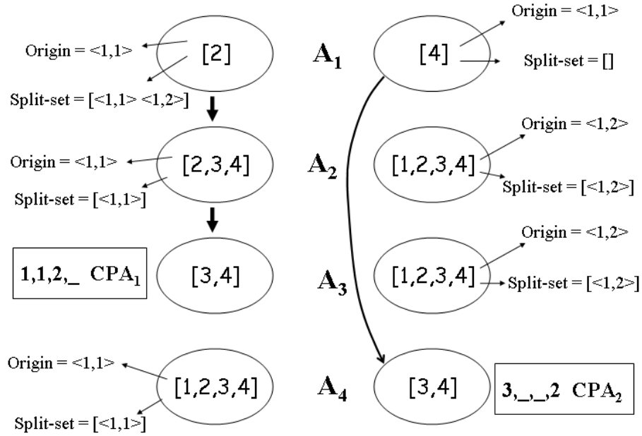
Figure 6: Simple Concurrent Search with two CPAs
