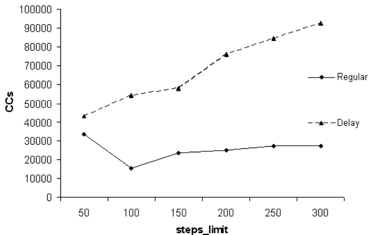
Figure 22: Number of non-concurrent constraint checks performed by ConcDB for a smaller range of steps_limits ( p_1 = 0.7 )
