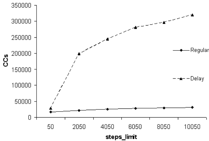
Figure 19: Number of non-concurrent constraint checks performed by ConcDB for increasing steps_limits ( p_1 = 0.4 )
